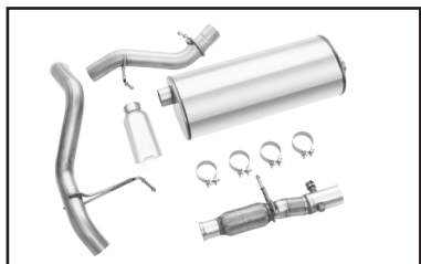
5.3L Single Exit Performance Exhaust
